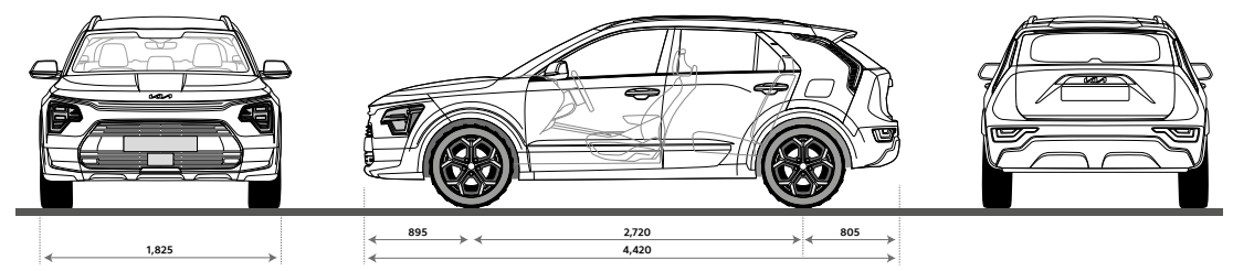
Dimensions Niro Hybride et Hybride Rechargeable (mm)
