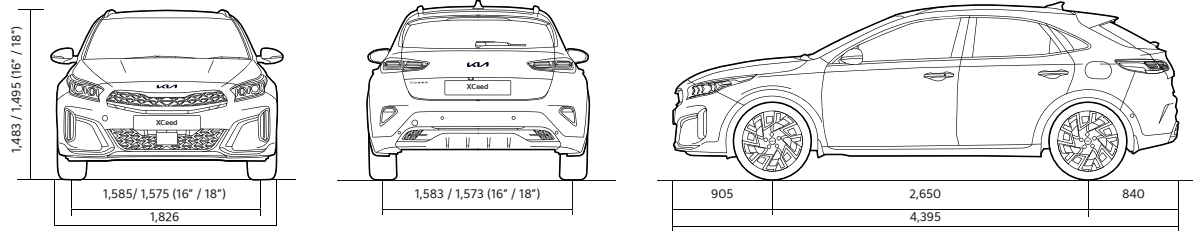
Dimensiones Drive / Tech (mm)
