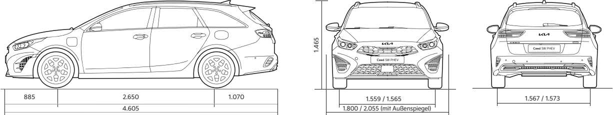
Abmessungen Ceed Sportswagon (in mm)
