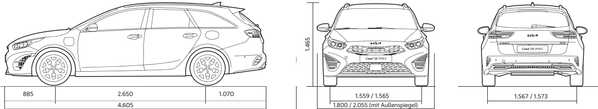
Abmessungen Ceed Sportswagon Plug-in Hybrid (in mm)
