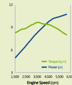
KAPPA 1.0 MPI ENGINE
