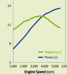
KAPPA 1.2 MPI ENGINE
